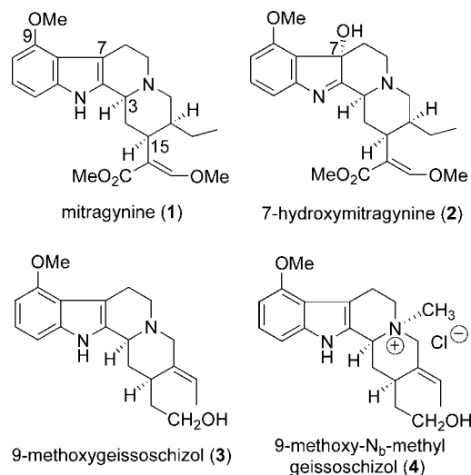
FIGURE 1. Structures of some 9-methoxy-substituted indole alkaloids.
