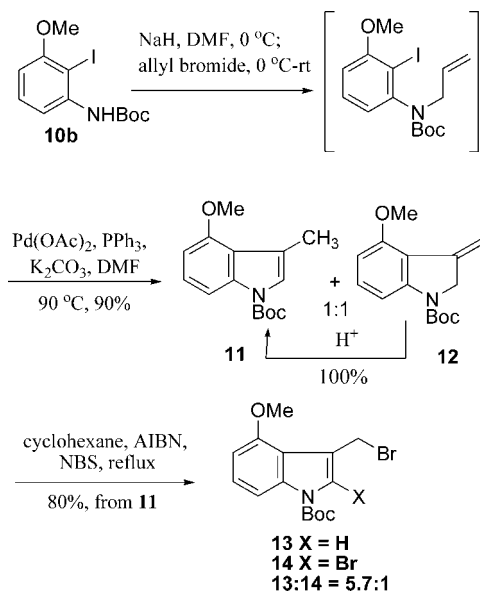
SCHEME 2. Initial Synthesis of Bromide 13
