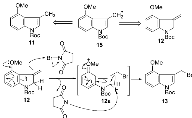
SCHEME 4. Improved Synthesis of Bromide 13 and Its Application in 4-Methoxytryptophan Synthesis
