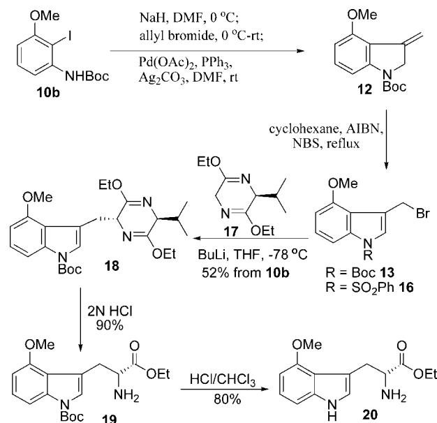
SCHEME 4. Improved Synthesis of Bromide 13 and Its Application in 4-Methoxytryptophan Synthesis
